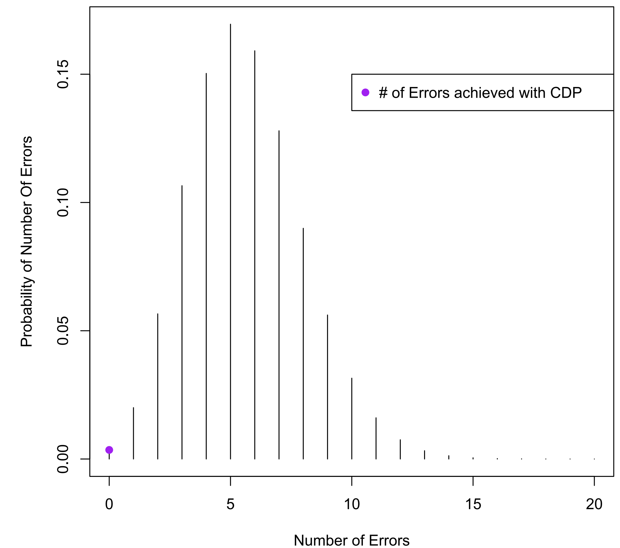
Plot 2: Binomial Distribution (n = 1126, p = .005)
